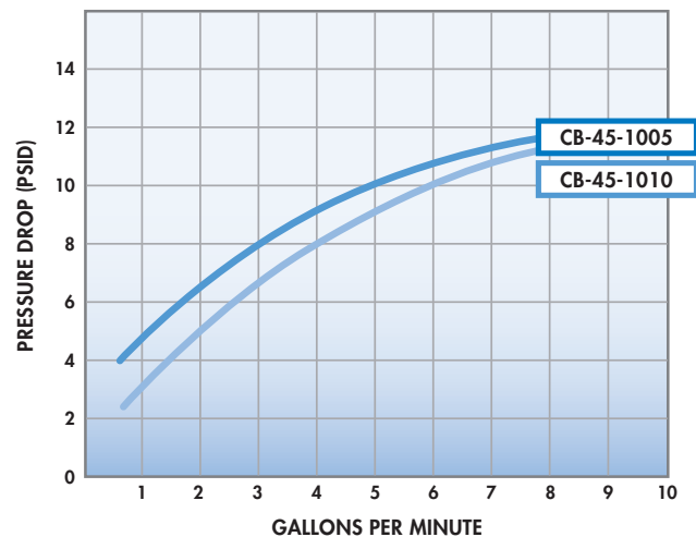
4.5" DIAMETER x 9 3/4" LENGTH
